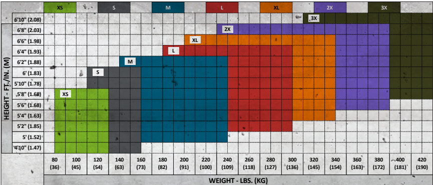
CHART 1: HARNESS SIZING
