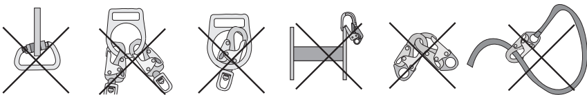
FIGURE 3: INAPPROPRIATE CONNECTIONS
