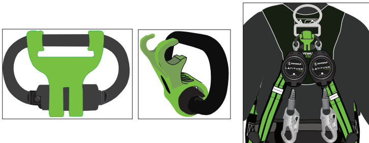
FIGURE 6: BEHIND THE WEB BRACKET INSTALLATION
