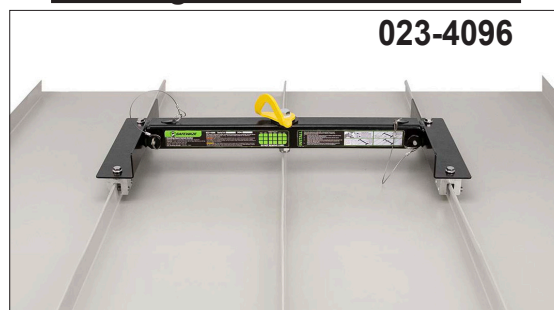
Standing Seam Swivel Anchor:
