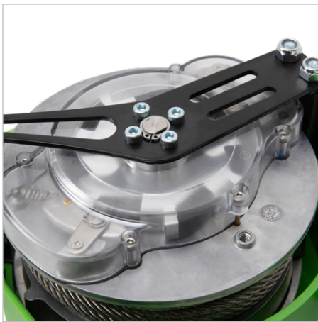
Longer product life with semi-sealed mainspring and pawl assembly
