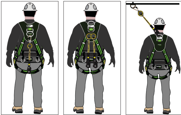
FIGURE 4: CONNECTION EXAMPLES
