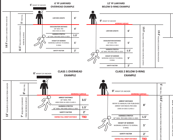
FIGURE 1: FALL CLEARANCE DIAGRAM
