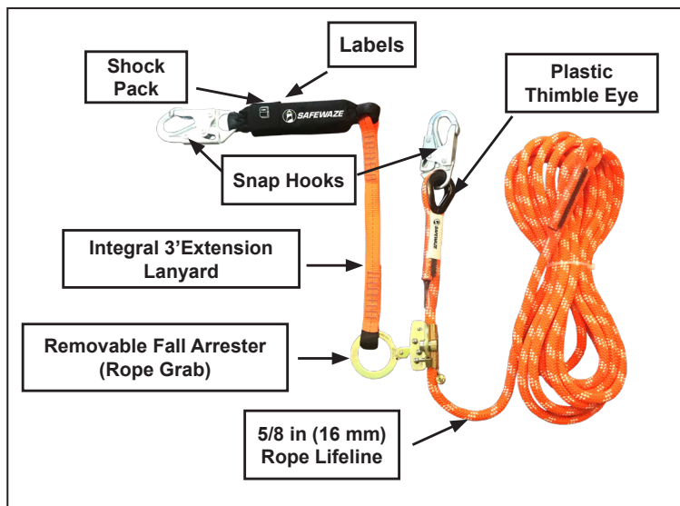
FIGURE 5 - COMPONENTS
