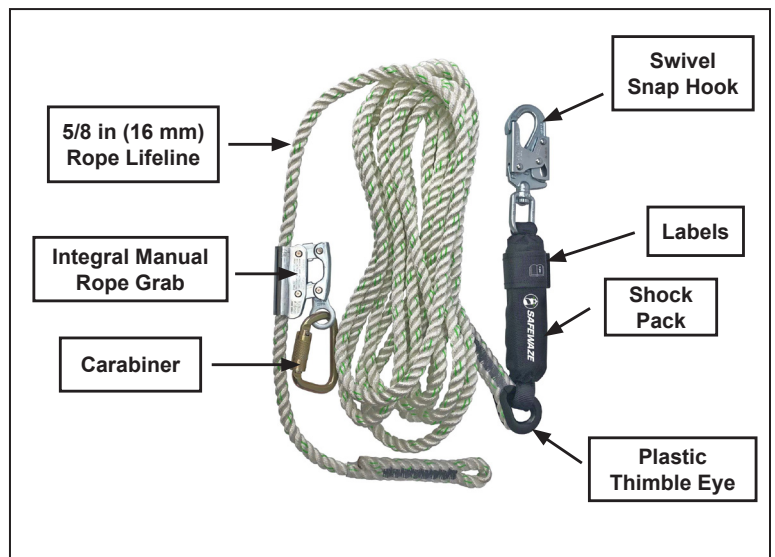
FIGURE 5 - COMPONENTS
