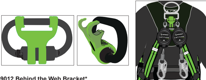
FIGURE 5: BEHIND THE WEB BRACKET INSTALLATION
