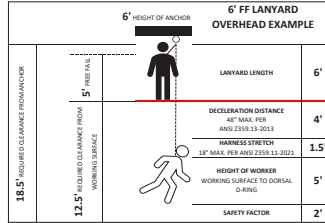
FIGURE 1: FALL CLEARANCE DIAGRAMS
