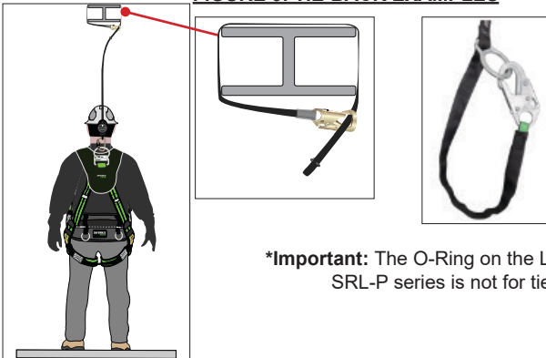
FIGURE 5: TIE-BACK EXAMPLES
