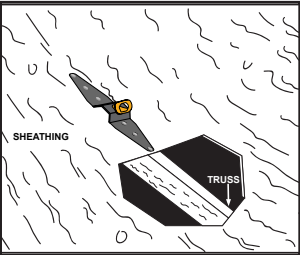
FIGURE 6B - CUT AWAY VIEW
