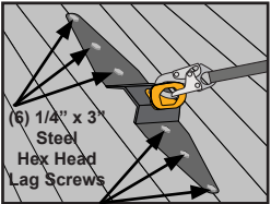
FIGURE 6B - CUT AWAY VIEW
