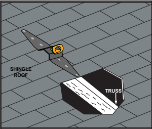
FIGURE 6C - CUT AWAY VIEW
