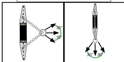
FIGURE 7 - ALLOWABLE WORK RADIUS
